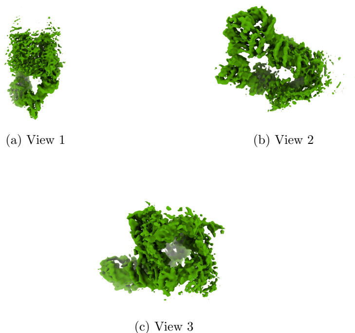
Figure 4: Isosurface at threshold=0.436000. Views generated by ChimeraX at a the following X, Y, Z angles: View 1 (0, -90, -90), View 2 (-90, 0, -90), View 3 (0, 0, 0).
