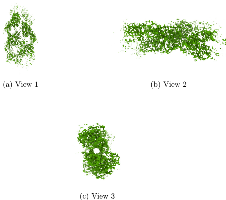
Figure 4: Isosurface at threshold=0.151000. Views generated by ChimeraX at a the following X, Y, Z angles: View 1 (0, -90, -90), View 2 (-90, 0, -90), View 3 (0, 0, 0).
