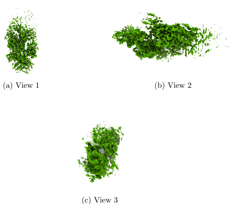
Figure 4: Isosurface at threshold=0.098000. Views generated by ChimeraX at a the following X, Y, Z angles: View 1 (0, -90, -90), View 2 (-90, 0, -90), View 3 (0, 0, 0).
