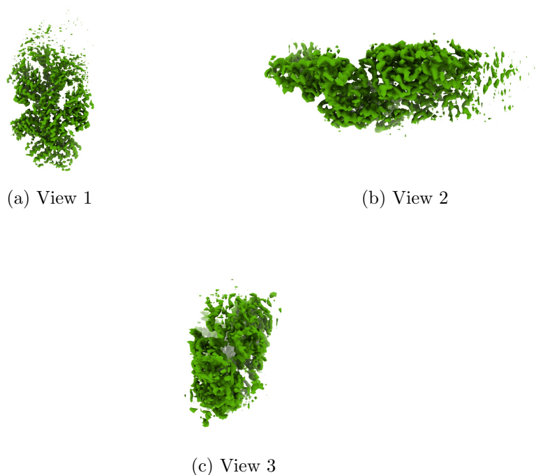
Figure 4: Isosurface at threshold=0.099600. Views generated by ChimeraX at a the following X, Y, Z angles: View 1 (0, -90, -90), View 2 (-90, 0, -90), View 3 (0, 0, 0).
