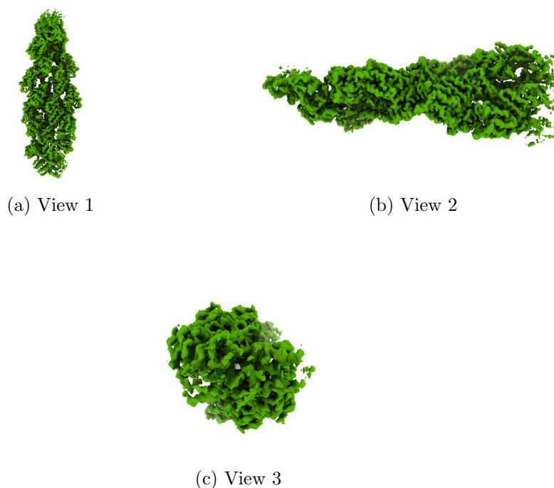
Figure 4: Isosurface at threshold=0.067300. Views generated by ChimeraX at a the following X, Y, Z angles: View 1 (0, -90, -90), View 2 (-90, 0, -90), View 3 (0, 0, 0).
