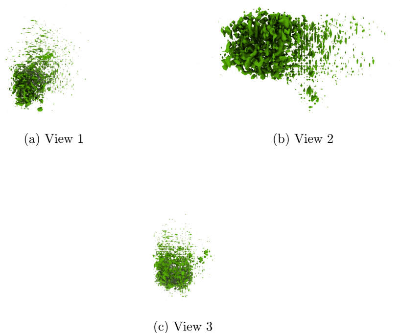
Figure 4: Isosurface at threshold=0.800000. Views generated by ChimeraX at a the following X, Y, Z angles: View 1 (0, -90, -90), View 2 (-90, 0, -90), View 3 (0, 0, 0).
