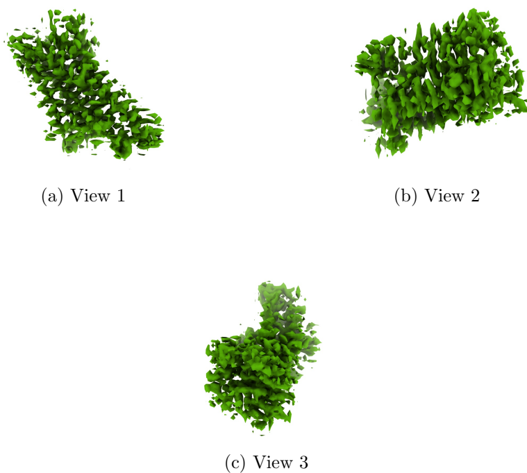
Figure 4: Isosurface at threshold=0.617000. Views generated by ChimeraX at a the following X, Y, Z angles: View 1 (0, -90, -90), View 2 (-90, 0, -90), View 3 (0, 0, 0).
