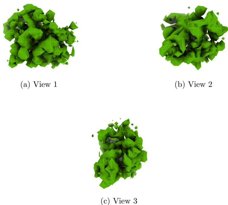
Figure 4: Isosurface at threshold=0.074800. Views generated by ChimeraX at a the following X, Y, Z angles: View 1 (0, -90, -90), View 2 (-90, 0, -90), View 3 (0, 0, 0).
