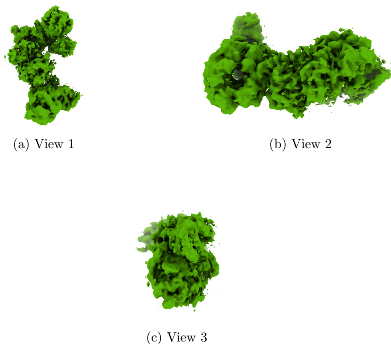
Figure 4: Isosurface at threshold=0.075200. Views generated by ChimeraX at a the following X, Y, Z angles: View 1 (0, -90, -90), View 2 (-90, 0, -90), View 3 (0, 0, 0).
