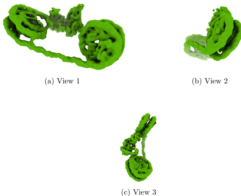
Figure 4: Isosurface at threshold=0.036600. Views generated by ChimeraX at a the following X, Y, Z angles: View 1 (0, -90, -90), View 2 (-90, 0, -90), View 3 (0, 0, 0).
