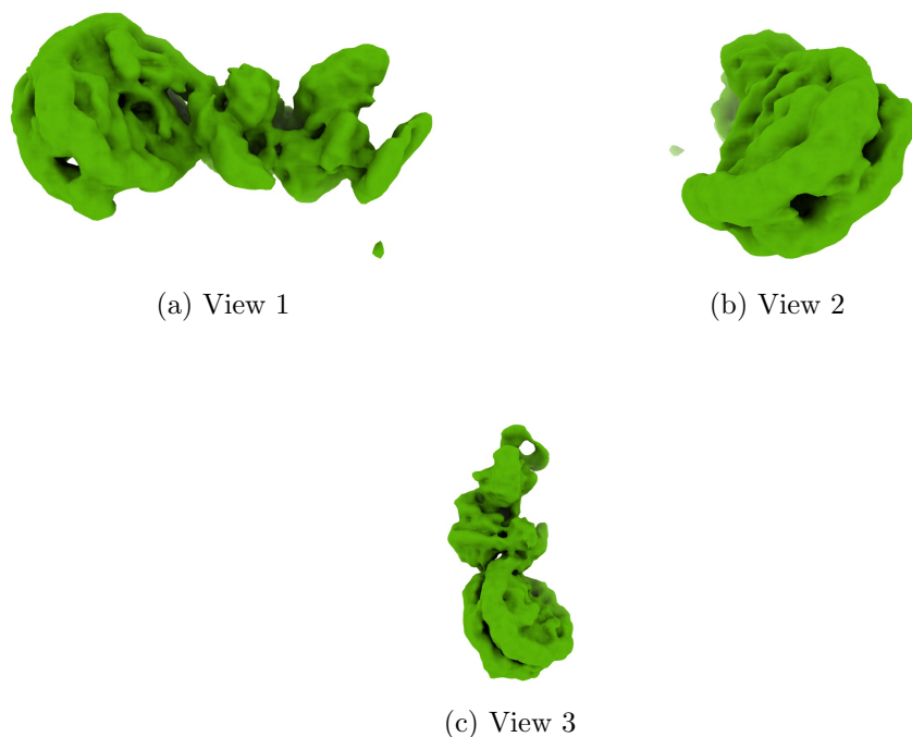
Figure 4: Isosurface at threshold=0.025000. Views generated by ChimeraX at a the following X, Y, Z angles: View 1 (0, -90, -90), View 2 (-90, 0, -90), View 3 (0, 0, 0).
