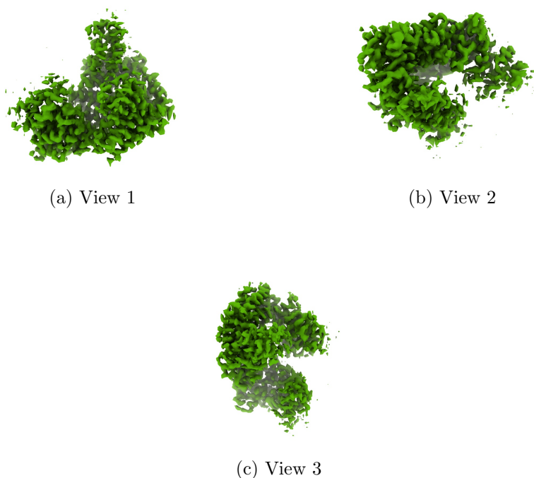
Figure 4: Isosurface at threshold=0.080000. Views generated by ChimeraX at a the following X, Y, Z angles: View 1 (0, -90, -90), View 2 (-90, 0, -90), View 3 (0, 0, 0).
