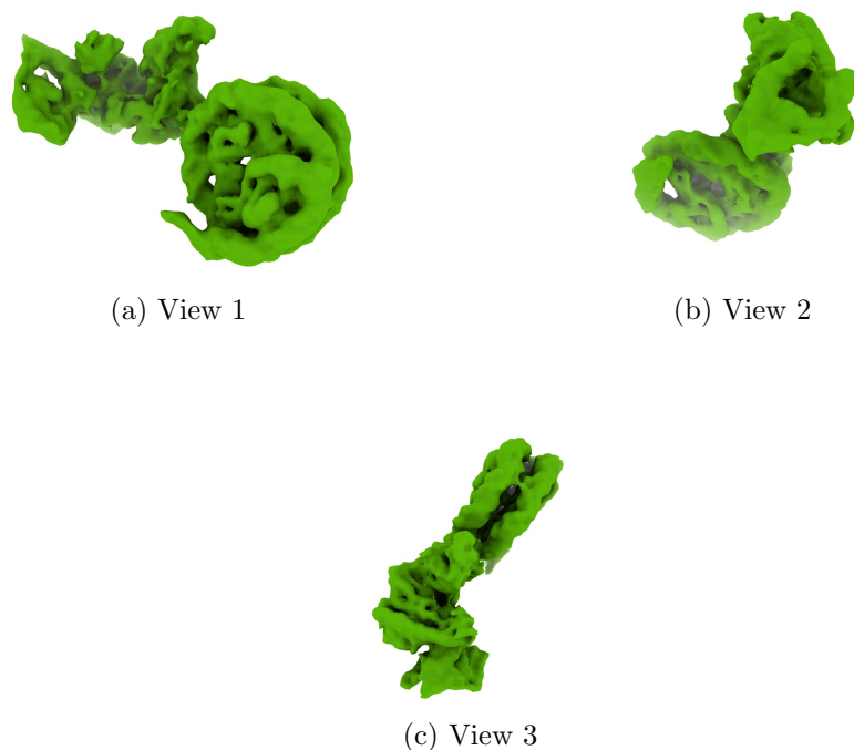
Figure 4: Isosurface at threshold=0.031000. Views generated by ChimeraX at a the following X, Y, Z angles: View 1 (0, -90, -90), View 2 (-90, 0, -90), View 3 (0, 0, 0).
