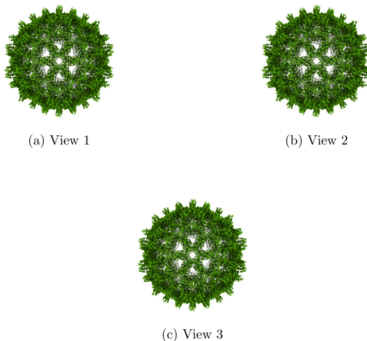
Figure 4: Isosurface at threshold=0.013100. Views generated by ChimeraX at a the following X, Y, Z angles: View 1 (0, -90, -90), View 2 (-90, 0, -90), View 3 (0, 0, 0).
