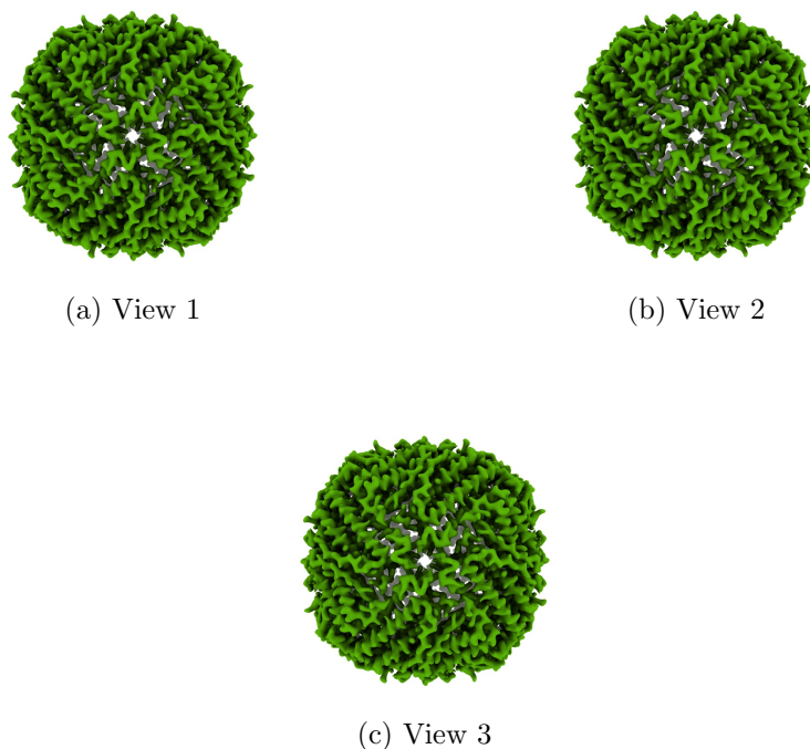
Figure 4: Isosurface at threshold=0.524000. Views generated by ChimeraX at a the following X, Y, Z angles: View 1 (0, -90, -90), View 2 (-90, 0, -90), View 3 (0, 0, 0).
