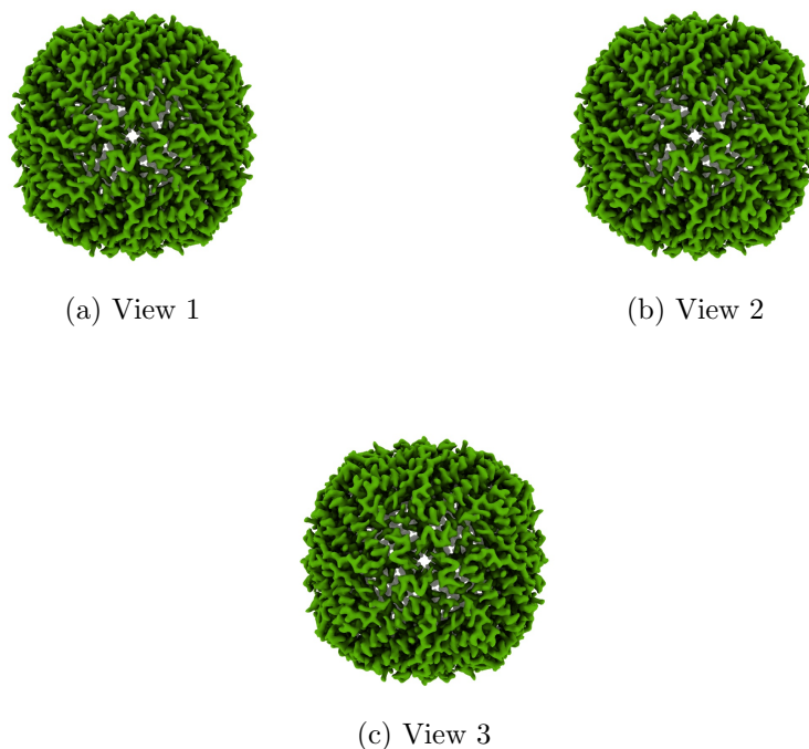
Figure 4: Isosurface at threshold=0.562000. Views generated by ChimeraX at a the following X, Y, Z angles: View 1 (0, -90, -90), View 2 (-90, 0, -90), View 3 (0, 0, 0).
