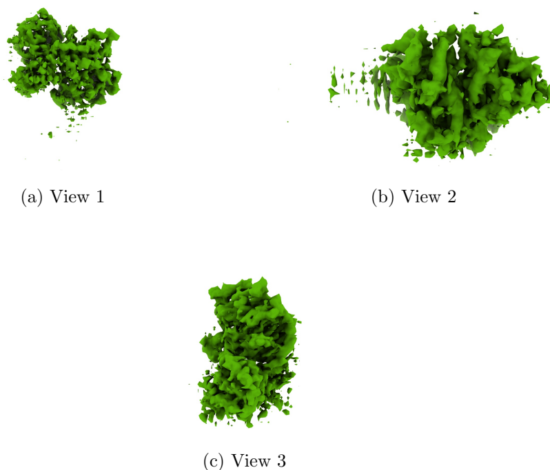
Figure 4: Isosurface at threshold=0.121000. Views generated by ChimeraX at a the following X, Y, Z angles: View 1 (0, -90, -90), View 2 (-90, 0, -90), View 3 (0, 0, 0).
