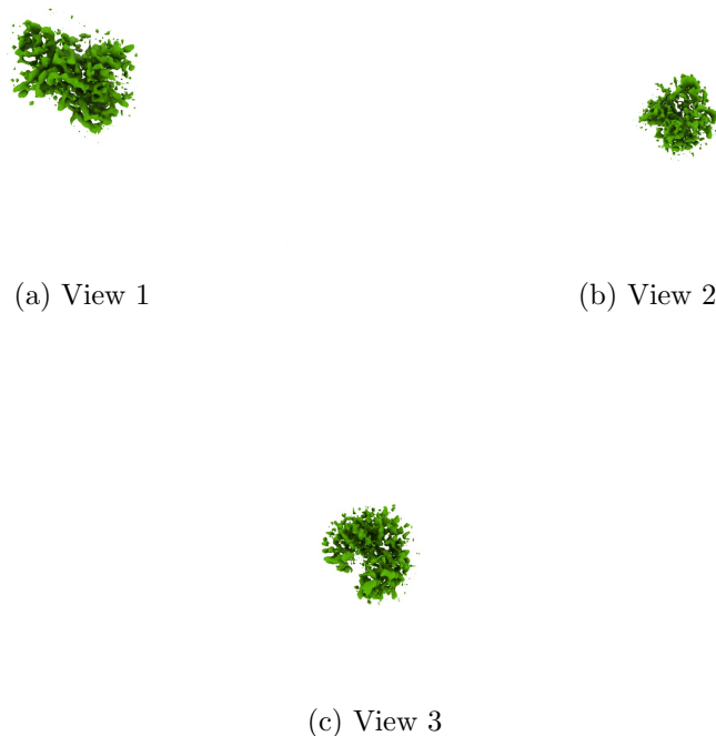
Figure 4: Isosurface at threshold=0.242000. Views generated by ChimeraX at a the following X, Y, Z angles: View 1 (0, -90, -90), View 2 (-90, 0, -90), View 3 (0, 0, 0).
