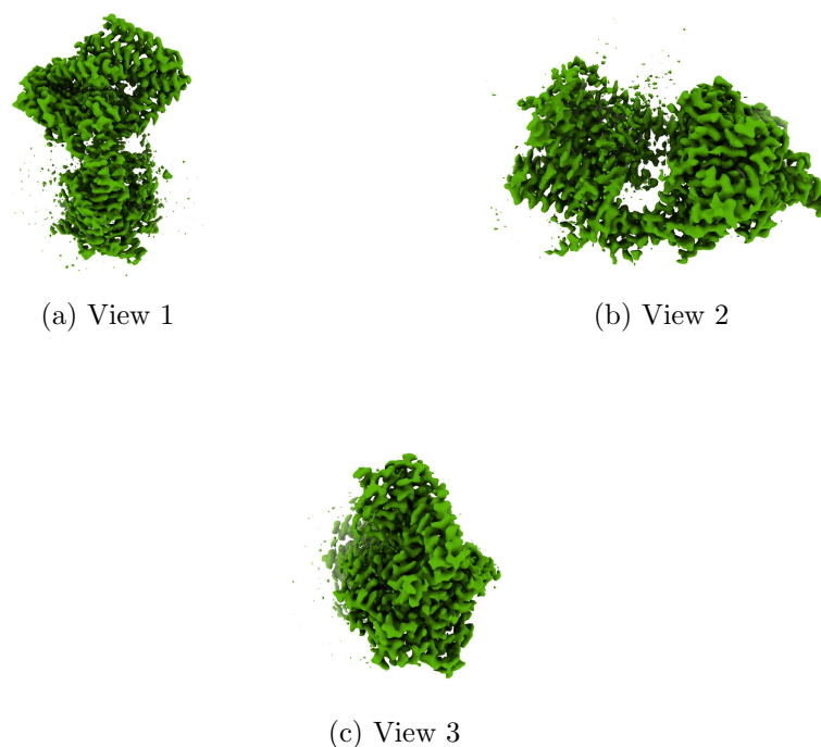
Figure 4: Isosurface at threshold=1.210000. Views generated by ChimeraX at a the following X, Y, Z angles: View 1 (0, -90, -90), View 2 (-90, 0, -90), View 3 (0, 0, 0).
