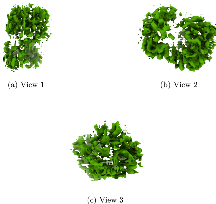
Figure 4: Isosurface at threshold=0.789000. Views generated by ChimeraX at a the following X, Y, Z angles: View 1 (0, -90, -90), View 2 (-90, 0, -90), View 3 (0, 0, 0).
