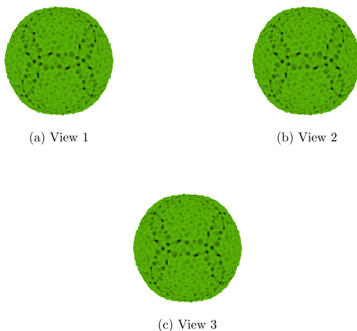
Figure 4: Isosurface at threshold=0.026700. Views generated by ChimeraX at a the following X, Y, Z angles: View 1 (0, -90, -90), View 2 (-90, 0, -90), View 3 (0, 0, 0).
