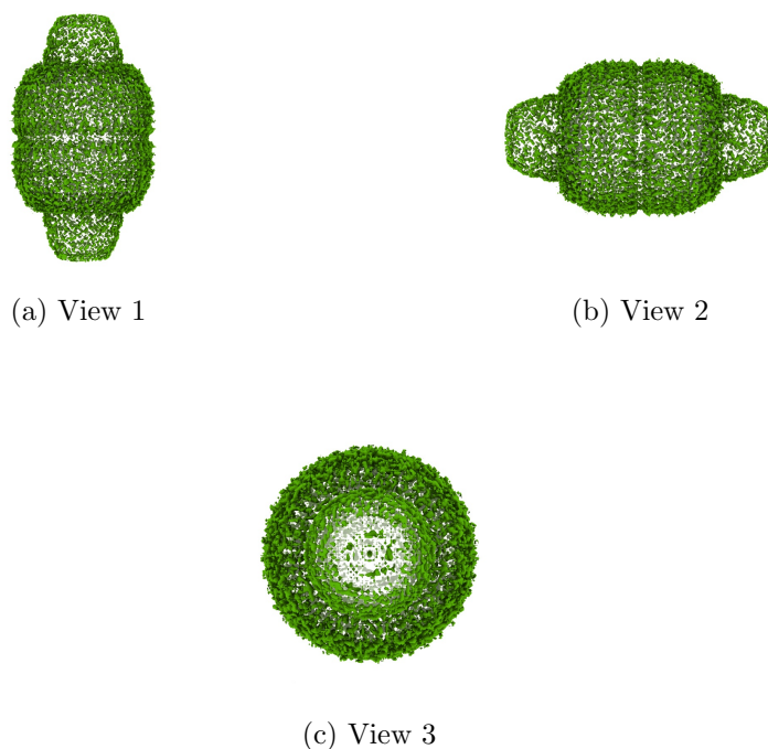
Figure 4: Isosurface at threshold=0.075300. Views generated by ChimeraX at a the following X, Y, Z angles: View 1 (0, -90, -90), View 2 (-90, 0, -90), View 3 (0, 0, 0).
