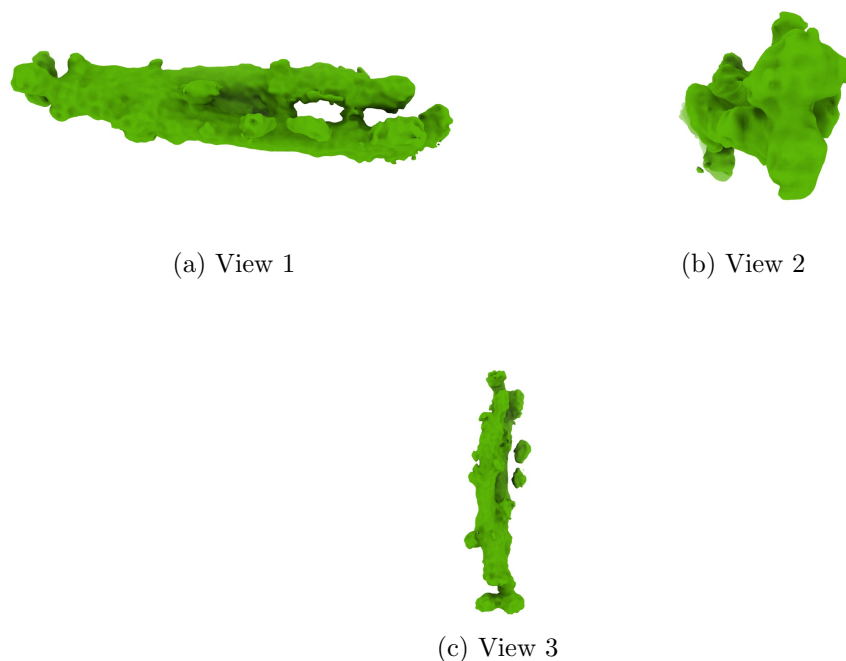
Figure 4: Isosurface at threshold=0.098300. Views generated by ChimeraX at a the following X, Y, Z angles: View 1 (0, -90, -90), View 2 (-90, 0, -90), View 3 (0, 0, 0).
