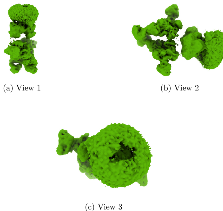
Figure 4: Isosurface at threshold=0.050000. Views generated by ChimeraX at a the following X, Y, Z angles: View 1 (0, -90, -90), View 2 (-90, 0, -90), View 3 (0, 0, 0).
