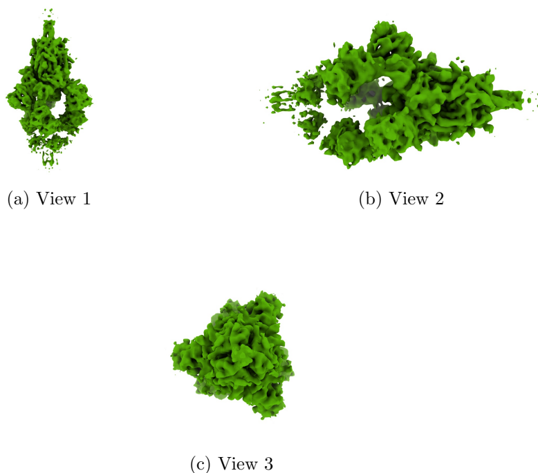
Figure 4: Isosurface at threshold=0.059800. Views generated by ChimeraX at a the following X, Y, Z angles: View 1 (0, -90, -90), View 2 (-90, 0, -90), View 3 (0, 0, 0).
