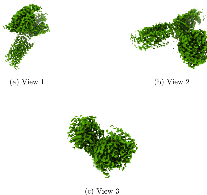
Figure 4: Isosurface at threshold=0.258000. Views generated by ChimeraX at a the following X, Y, Z angles: View 1 (0, -90, -90), View 2 (-90, 0, -90), View 3 (0, 0, 0).
