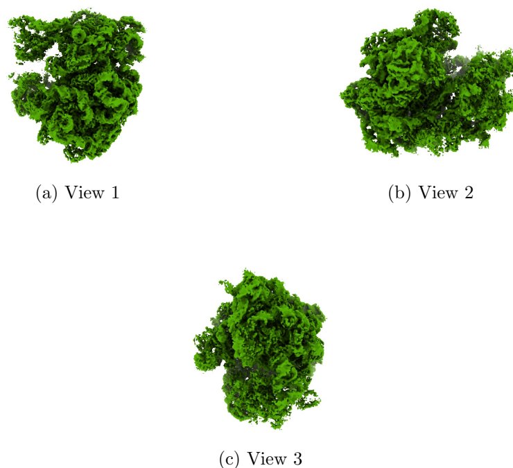
Figure 4: Isosurface at threshold=0.024500. Views generated by ChimeraX at a the following X, Y, Z angles: View 1 (0, -90, -90), View 2 (-90, 0, -90), View 3 (0, 0, 0).
