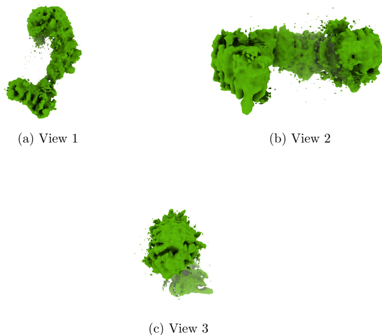
Figure 4: Isosurface at threshold=0.275000. Views generated by ChimeraX at a the following X, Y, Z angles: View 1 (0, -90, -90), View 2 (-90, 0, -90), View 3 (0, 0, 0).
