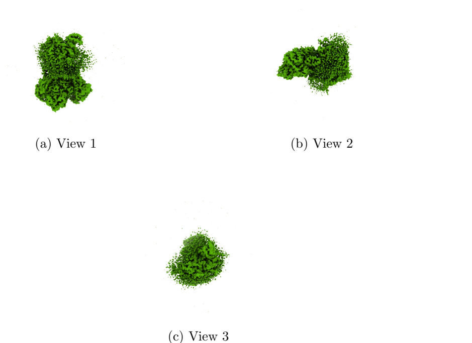
Figure 4: Isosurface at threshold=0.400000. Views generated by ChimeraX at a the following X, Y, Z angles: View 1 (0, -90, -90), View 2 (-90, 0, -90), View 3 (0, 0, 0).
