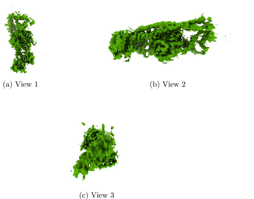
Figure 4: Isosurface at threshold=0.220000. Views generated by ChimeraX at a the following X, Y, Z angles: View 1 (0, -90, -90), View 2 (-90, 0, -90), View 3 (0, 0, 0).
