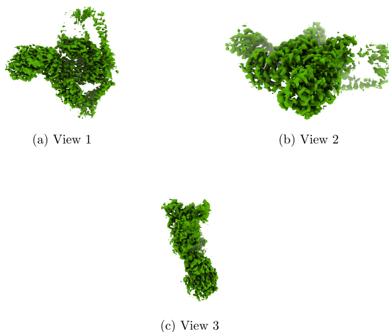
Figure 4: Isosurface at threshold=0.220000. Views generated by ChimeraX at a the following X, Y, Z angles: View 1 (0, -90, -90), View 2 (-90, 0, -90), View 3 (0, 0, 0).
