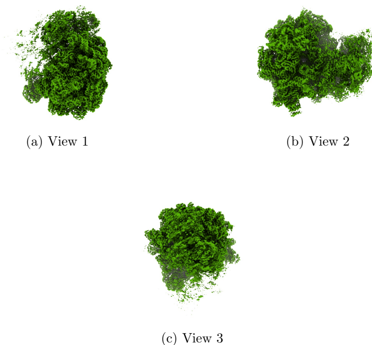
Figure 4: Isosurface at threshold=0.089900. Views generated by ChimeraX at a the following X, Y, Z angles: View 1 (0, -90, -90), View 2 (-90, 0, -90), View 3 (0, 0, 0).
