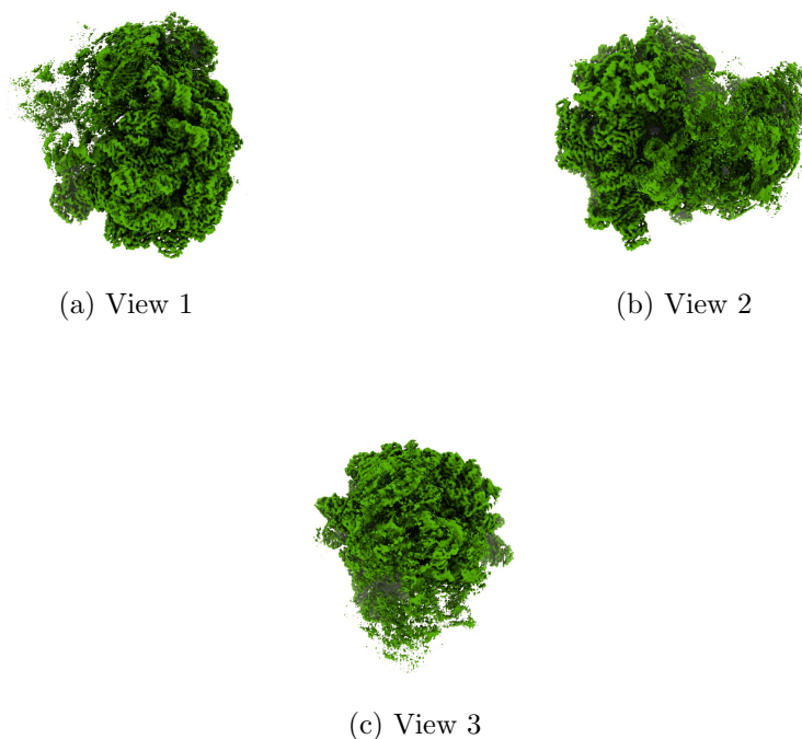
Figure 4: Isosurface at threshold=0.075700. Views generated by ChimeraX at a the following X, Y, Z angles: View 1 (0, -90, -90), View 2 (-90, 0, -90), View 3 (0, 0, 0).
