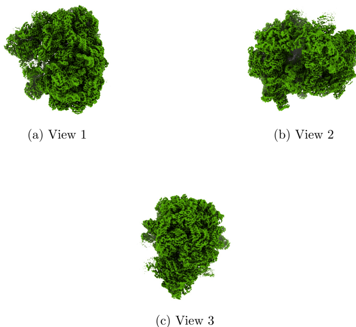
Figure 4: Isosurface at threshold=0.059200. Views generated by ChimeraX at a the following X, Y, Z angles: View 1 (0, -90, -90), View 2 (-90, 0, -90), View 3 (0, 0, 0).
