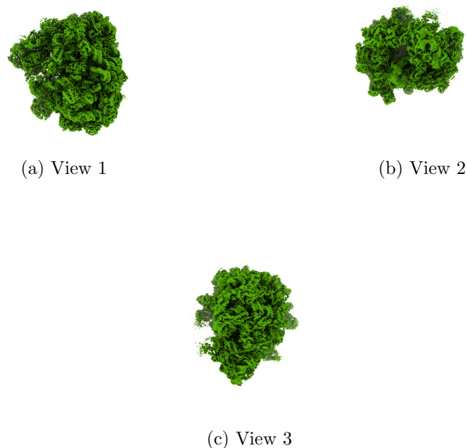
Figure 4: Isosurface at threshold=0.052500. Views generated by ChimeraX at a the following X, Y, Z angles: View 1 (0, -90, -90), View 2 (-90, 0, -90), View 3 (0, 0, 0).
