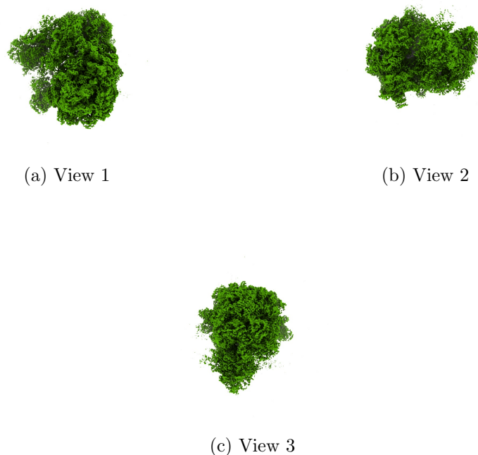
Figure 4: Isosurface at threshold=0.073100. Views generated by ChimeraX at a the following X, Y, Z angles: View 1 (0, -90, -90), View 2 (-90, 0, -90), View 3 (0, 0, 0).
