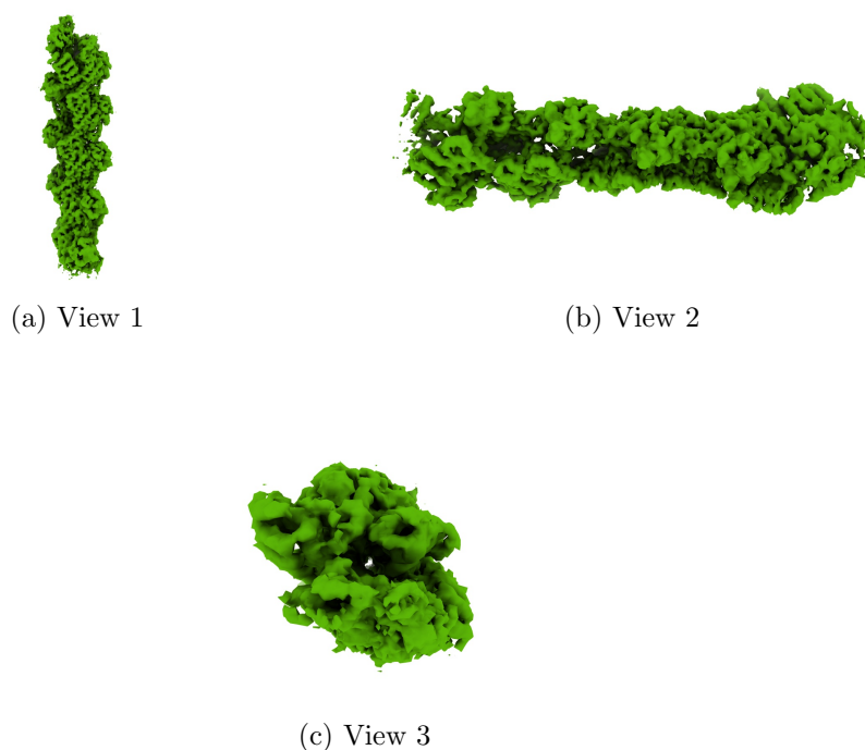
Figure 4: Isosurface at threshold=0.143000. Views generated by ChimeraX at a the following X, Y, Z angles: View 1 (0, -90, -90), View 2 (-90, 0, -90), View 3 (0, 0, 0).
