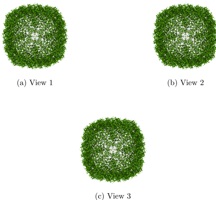
Figure 4: Isosurface at threshold=0.103000. Views generated by ChimeraX at the following X, Y, Z angles: View 1 (0, -90, -90), View 2 (-90, 0, -90), View 3 (0, 0, 0).
