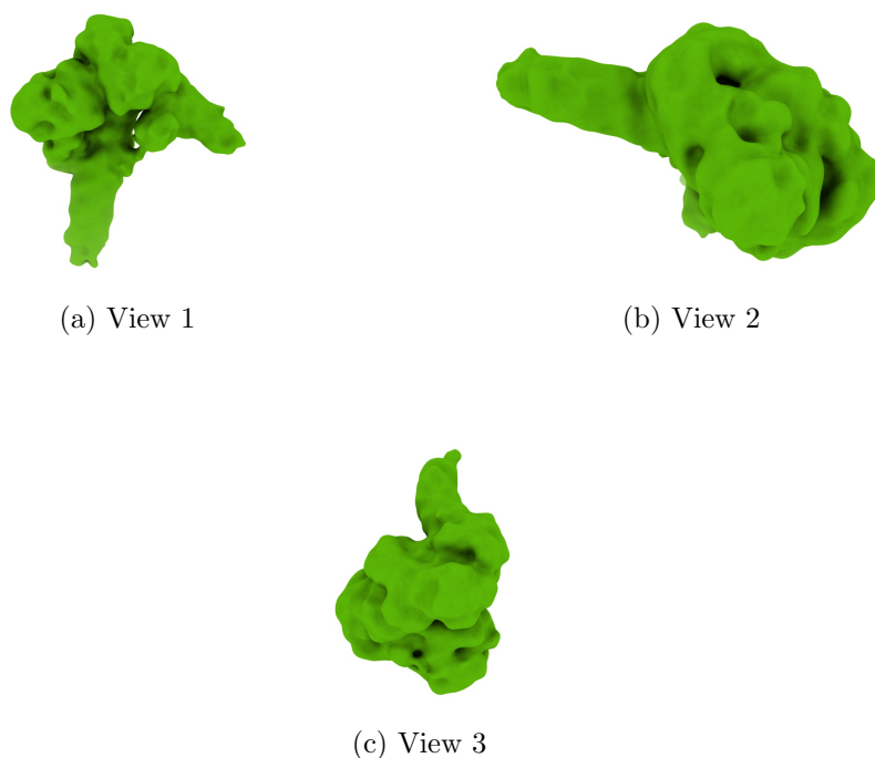
Figure 4: Isosurface at threshold=0.007030. Views generated by ChimeraX at a the following X, Y, Z angles: View 1 (0, -90, -90), View 2 (-90, 0, -90), View 3 (0, 0, 0).
