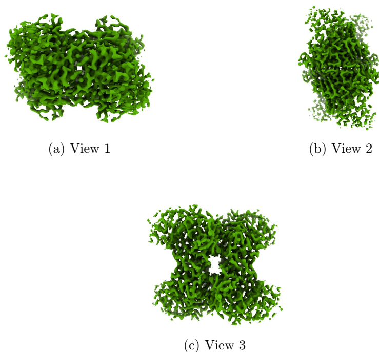
Figure 4: Isosurface at threshold=1.120000. Views generated by ChimeraX at a the following X, Y, Z angles: View 1 (0, -90, -90), View 2 (-90, 0, -90), View 3 (0, 0, 0).
