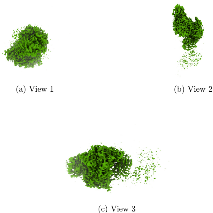
Figure 4: Isosurface at threshold=0.080000. Views generated by ChimeraX at a the following X, Y, Z angles: View 1 (0, -90, -90), View 2 (-90, 0, -90), View 3 (0, 0, 0).
