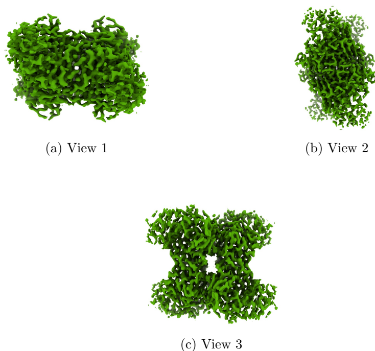
Figure 4: Isosurface at threshold=0.963000. Views generated by ChimeraX at a the following X, Y, Z angles: View 1 (0, -90, -90), View 2 (-90, 0, -90), View 3 (0, 0, 0).
