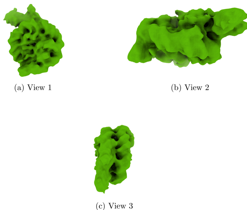
Figure 4: Isosurface at threshold=0.282000. Views generated by ChimeraX at a the following X, Y, Z angles: View 1 (0, -90, -90), View 2 (-90, 0, -90), View 3 (0, 0, 0).
