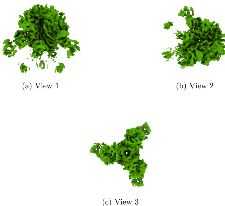
Figure 4: Isosurface at threshold=0.381000. Views generated by ChimeraX at a the following X, Y, Z angles: View 1 (0, -90, -90), View 2 (-90, 0, -90), View 3 (0, 0, 0).
