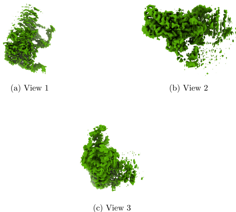
Figure 4: Isosurface at threshold=8.000000. Views generated by ChimeraX at a the following X, Y, Z angles: View 1 (0, -90, -90), View 2 (-90, 0, -90), View 3 (0, 0, 0).
