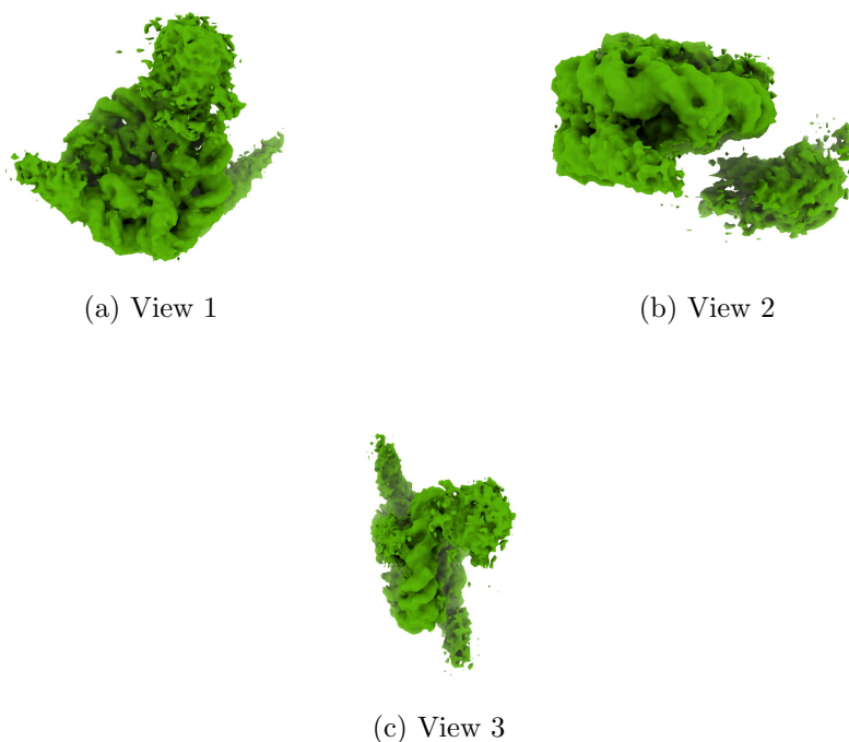
Figure 4: Isosurface at threshold=0.077200. Views generated by ChimeraX at a the following X, Y, Z angles: View 1 (0, -90, -90), View 2 (-90, 0, -90), View 3 (0, 0, 0).
