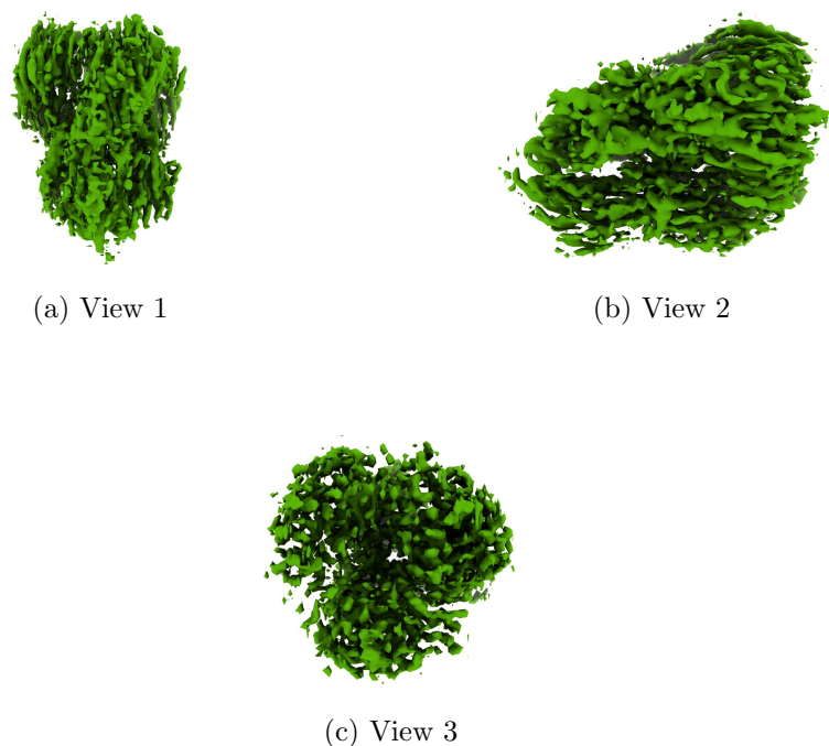
Figure 4: Isosurface at threshold=0.031100. Views generated by ChimeraX at a the following X, Y, Z angles: View 1 (0, -90, -90), View 2 (-90, 0, -90), View 3 (0, 0, 0).
