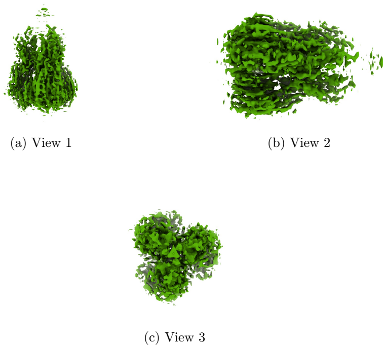
Figure 4: Isosurface at threshold=0.040200. Views generated by ChimeraX at a the following X, Y, Z angles: View 1 (0, -90, -90), View 2 (-90, 0, -90), View 3 (0, 0, 0).
