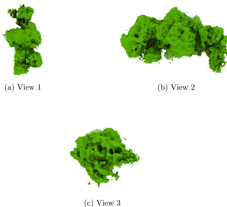
Figure 4: Isosurface at threshold=0.033700. Views generated by ChimeraX at a the following X, Y, Z angles: View 1 (0, -90, -90), View 2 (-90, 0, -90), View 3 (0, 0, 0).
