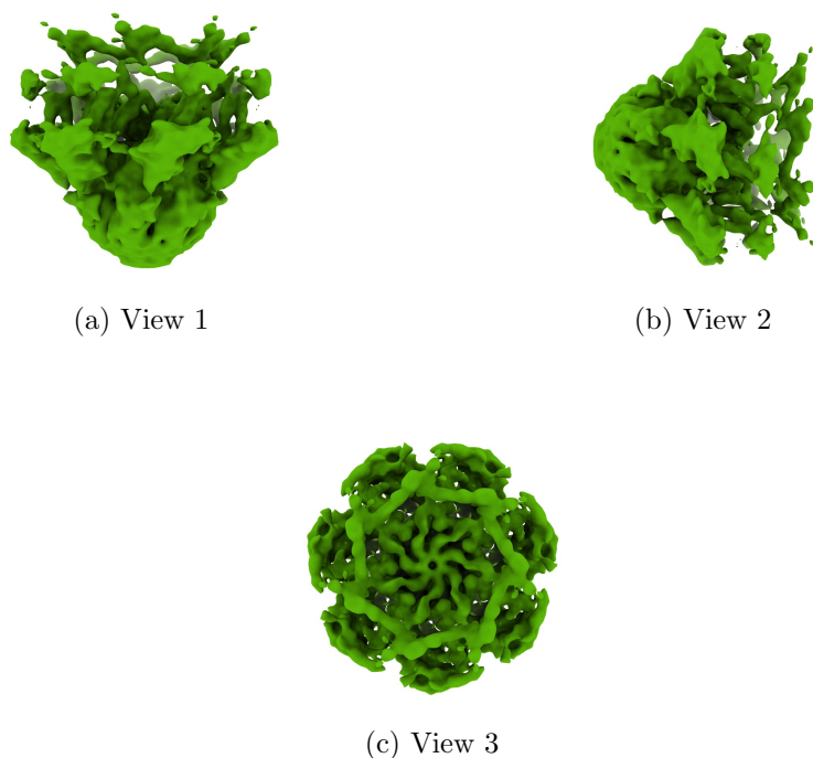
Figure 4: Isosurface at threshold=0.091000. Views generated by ChimeraX at a the following X, Y, Z angles: View 1 (0, -90, -90), View 2 (-90, 0, -90), View 3 (0, 0, 0).
